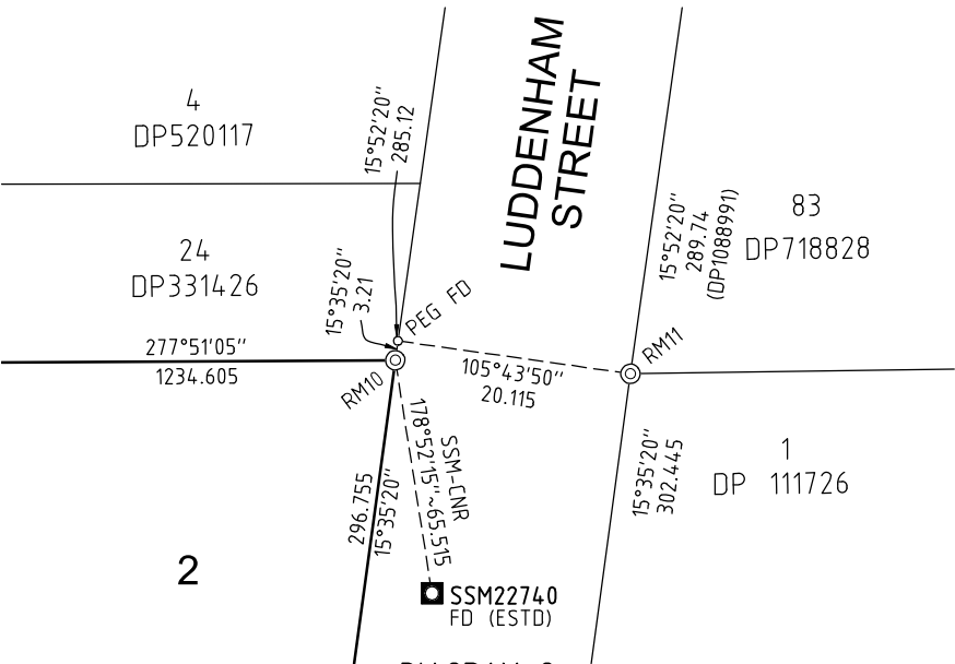
DIAGRAM 2 SCALE 1:1000
