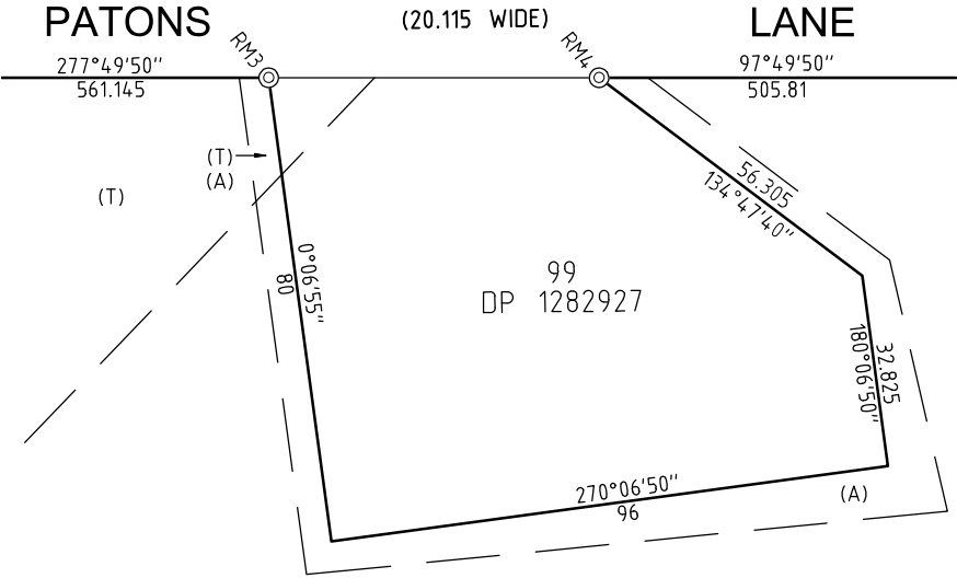
DIAGRAM 1 SCALE 1:1000
